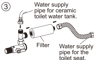
Water pipe valve connected to T valve.
